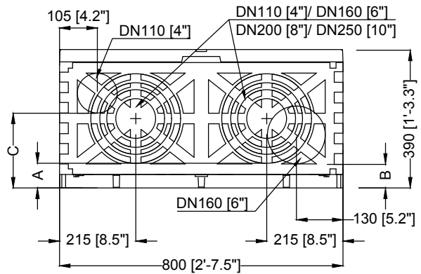
EcoBloc light system 402301 + 402300 + 402303
